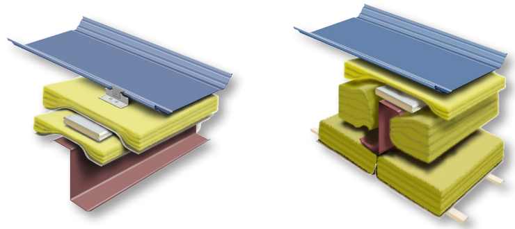
The SNS ® Thermal Block "The Performer" comes in six-foot lengths. Each SSR Panel Clip is placed on top of the SNS ® Thermal Block "The Performer" and will be fastened through the block and attached to the purlin flange for a tight connection. They are designed to resist normal vertical and horizontal loads applied in a typical metal building application.
